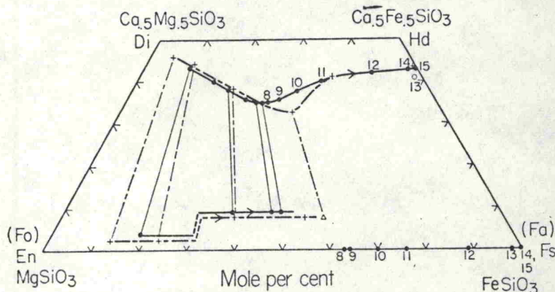
Fig. 1. Trends of pyroxene compositions for the Skaergaard and Bushveld intrusions. Skaergaard: solid circles, compositions of analyzed pyroxenes; open circle, composition of analyzed inverted ferriiferous wollastonite; heavy solid lines, trends of Ca-rich and Ca-poor pyroxenes; light solid lines, tie lines between coexisting pyroxenes (Brown, 1957; Brown and Vincent, 1963). Dots along Fs-En join give Fe/Mg ratios of olivines coexisting with similarly-numbered Ca-rich pyroxenes from the Skaergaard intrusion. Bushveld: crosses, analyzed pyroxenes; triangle, composition of latest cumulus Ca-poor pyroxene (optical determination); heavy dash-dot lines, trends of Ca-rich and Ca-poor pyroxenes; light dash-dot lines, tie lines between coexisting pyroxenes (Atkins, quoted in Wager and Brown, 1968). Dashed lines, compositional breaks between orthopyroxenes and pigeonites. Arrows show direction of progressive crystallization.
