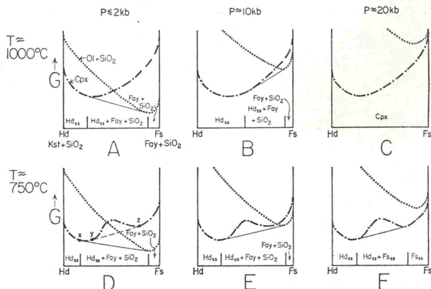
Fig 4. Schematic free energy-composition diagrams plotted as a function of 3 pressures for temperatures of 1000°C and 750°C. Dash-dot lines: free energy for clinopyroxene solid solutions; dotted lines: free energy for equimolar olivine + \text{SiO}_2 mixtures. Polymorphism in ferrosilite is not considered. Solid tangent lines connect coexisting stable phases, and dashed tangent line (y-z in D) connects two coexisting metastable clinopyroxenes. The high temperature sections (A-C) show the effect of pressure on increasing the solubility of \text{FeSiO}_3 in \text{Ca}_{0.5}\text{Fe}_{0.5}\text{SiO}_3 ; at 20 kb there is complete solid solution along the join. At lower temperatures (D-F) a miscibility gap in the clinopyroxene series is assumed to exist. This miscibility gap is metastable at low pressures (D, E) but becomes stable at high pressures (F). From (D) it is obvious that at low pressures the metastable miscibility gap (y-z) must always be to the right of the stable curve defining the composition (x) of \text{Hd}_{ss} in equilibrium with \text{Fay} + \text{SiO}_2 . Note that it is impossible to demonstrate the existence of a metastable miscibility gap at low pressures inasmuch as the stable assemblages shown in A and D are identical.
