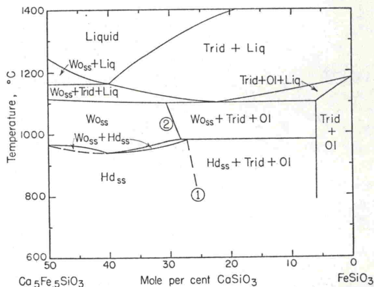
Fig. 2. The join hedenbergite-ferrosilite at 1 atm, after Bowen, Schairer, and Posnjak (1933, fig. 8). The liquids contain a small amount of Fe 2 O 3 . All phases are in equilibrium with metallic iron. Note the minimum in the inversion loop for Hd ss -Wo ss . Curves (1) and (2) are discussed in the text. Liq, liquid; trid, tridymite; Fay, Fe 2 SiO 4 -rich olivine; Wo ss , Fe-wollastonite solid solutions; Hd ss , hedenbergite solid solutions.
